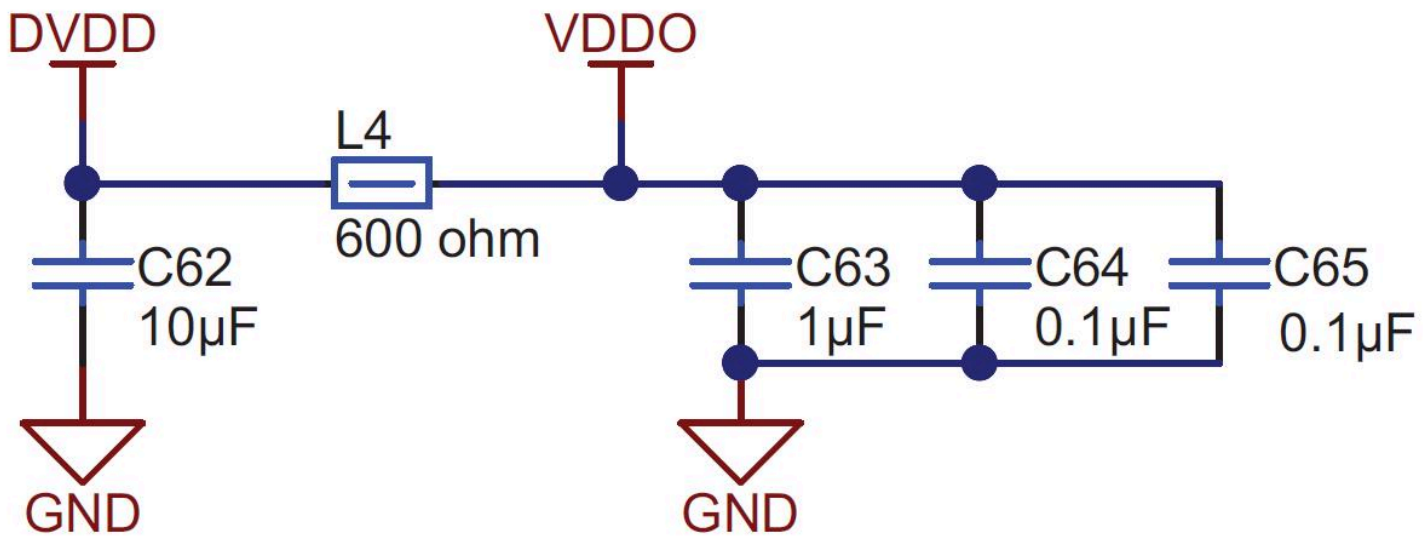
Figure 7. Decoupling components (capacitors and ferrite) for the ADC digital supply (DVDD) and clock buffer output supply (VDDO) on the ADS127L01EVM schematic
