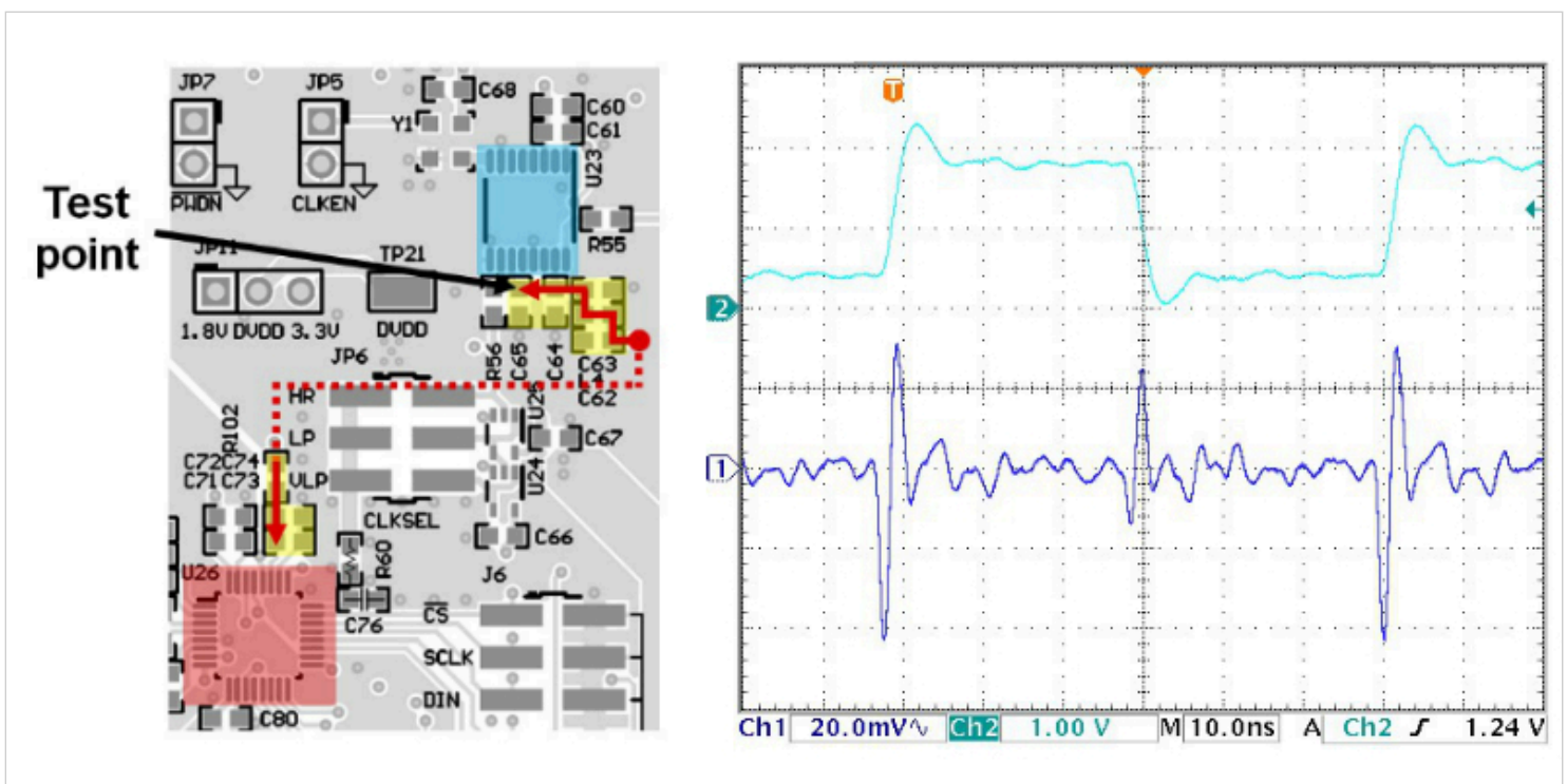
Figure 8. ADS127L01EVM schematic (left) and voltage measurements at buffer test point (right)
