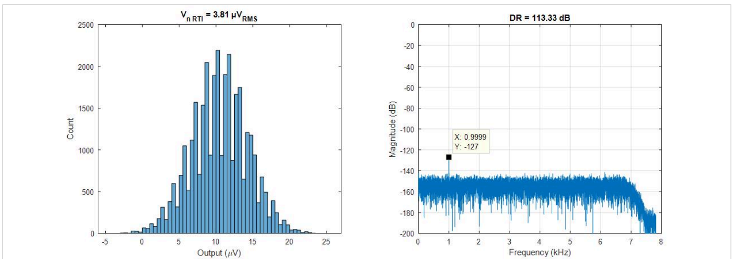
Figure 3. Noise histogram (left) and FFT (right) for clean supplies on LVDD and DVDD, ripple on AVDD
