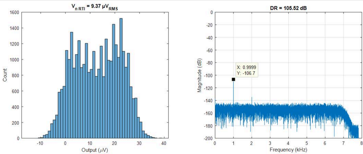
Figure 4. Noise histogram (left) and FFT (right) for clean supplies on AVDD and DVDD, ripple on LVDD
