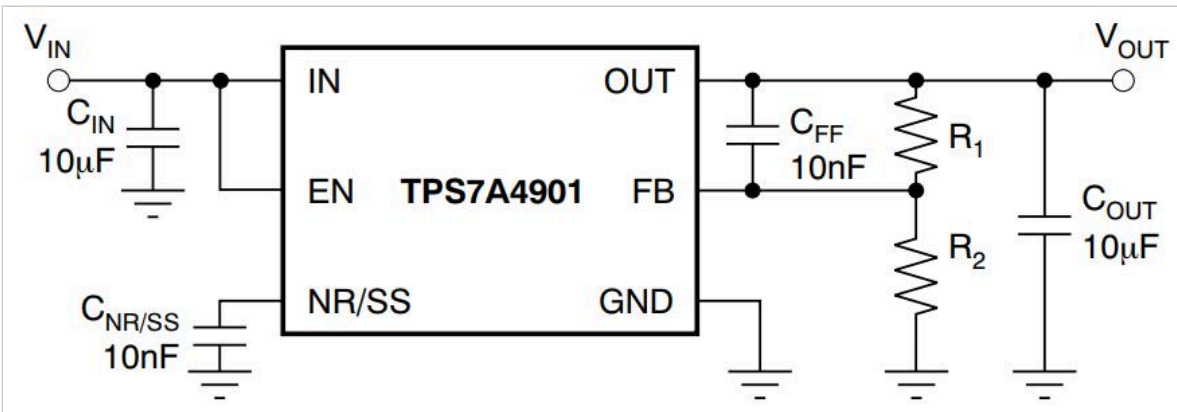
Figure 13. Filtering capacitors on an LDO
