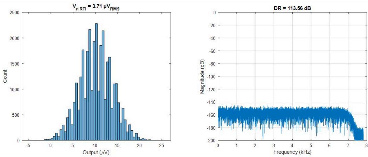
Figure 2. Noise histogram (left) and FFT (right) for clean supplies on AVDD, LVDD, and DVDD
