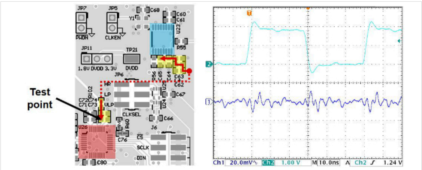
Figure 9. ADS127L01EVM schematic (left) and voltage measurements at ADC test point (right)
