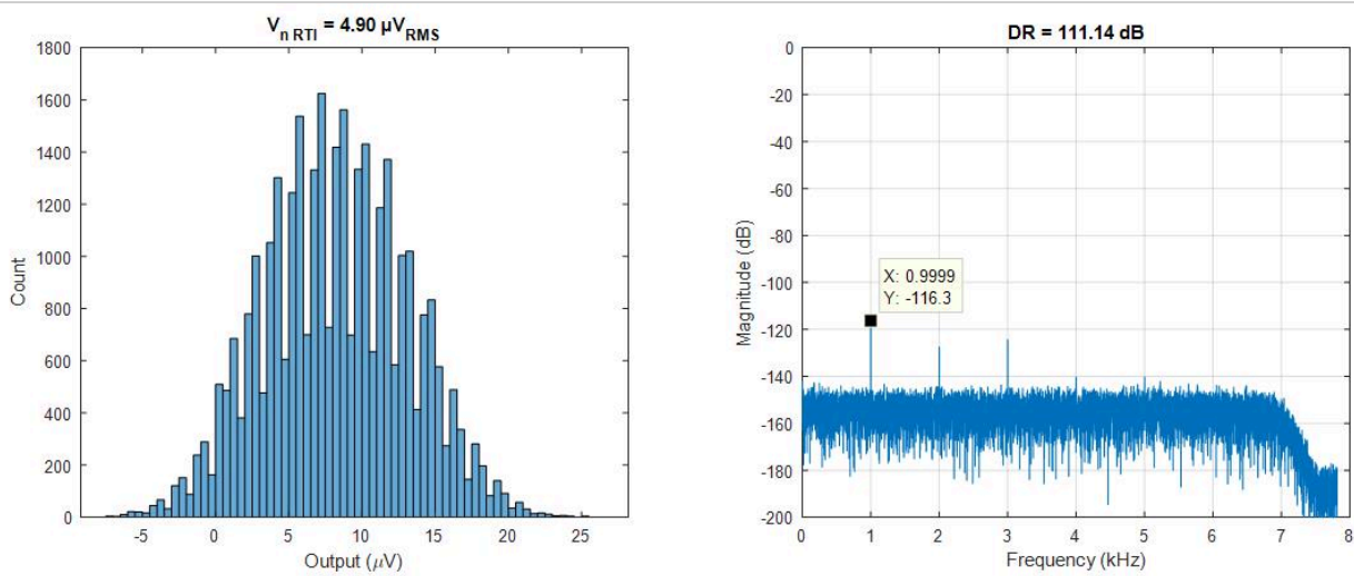
Figure 5. Noise histogram (left) and FFT (right) for clean supplies on AVDD and LVDD, ripple on DVDD
