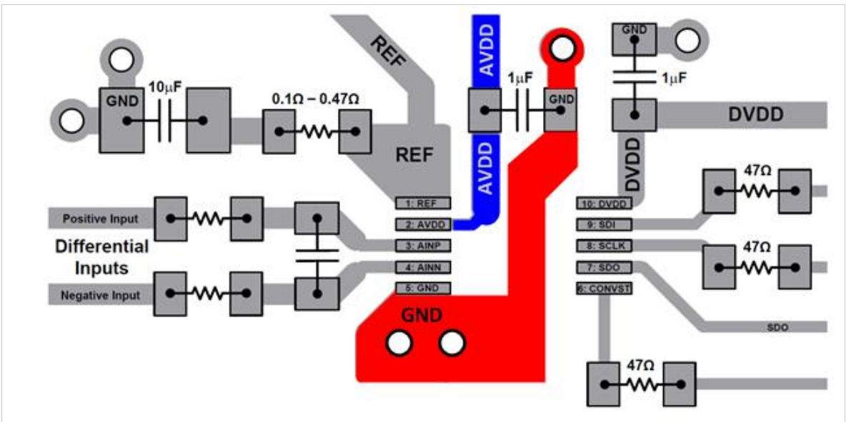
Figure 10. Routing techniques including thick traces and routing through capacitor pads
