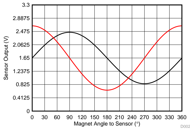
Figure 10. Two Sensors 90° Apart Uncalibrated Data
