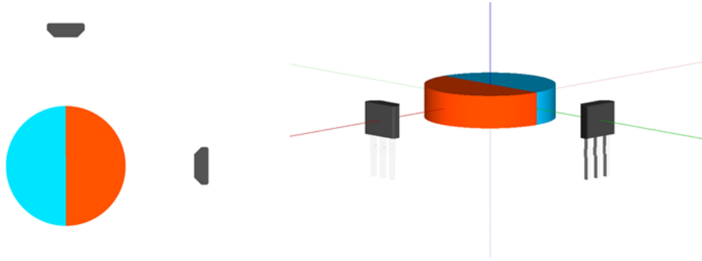
Figure 9. Two Sensors 90° Apart
