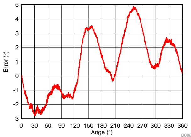
Figure 18. Two Sensors Peak Calibrated Error
