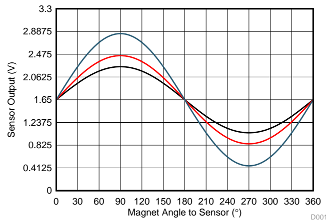
Figure 8. One Sensor Uncalibrated Data
