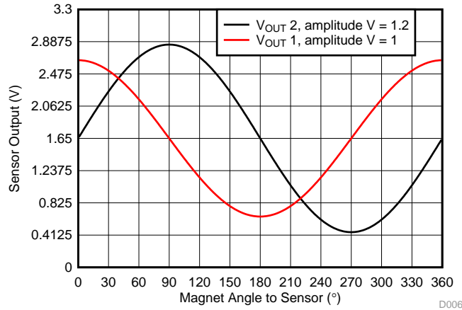
Figure 17. Two Sensors Peak Calibrated Data
