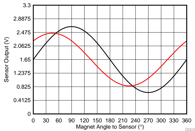
Figure 12. Two Sensors 45^\circ Apart Uncalibrated Data
