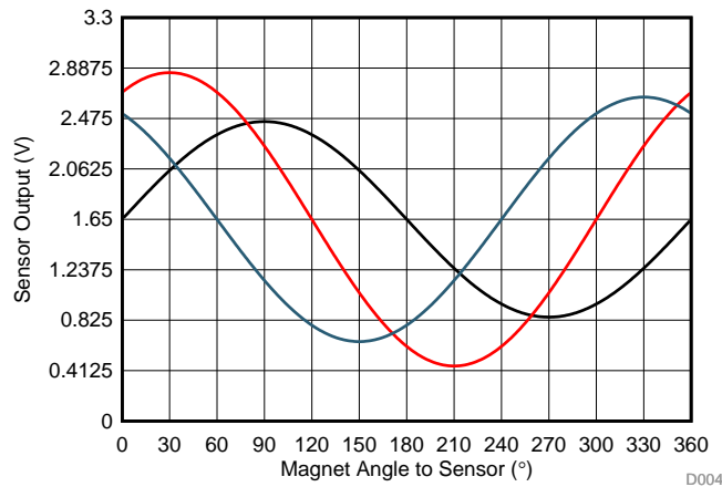
Figure 14. Three Sensors 60° Apart Uncalibrated Data
