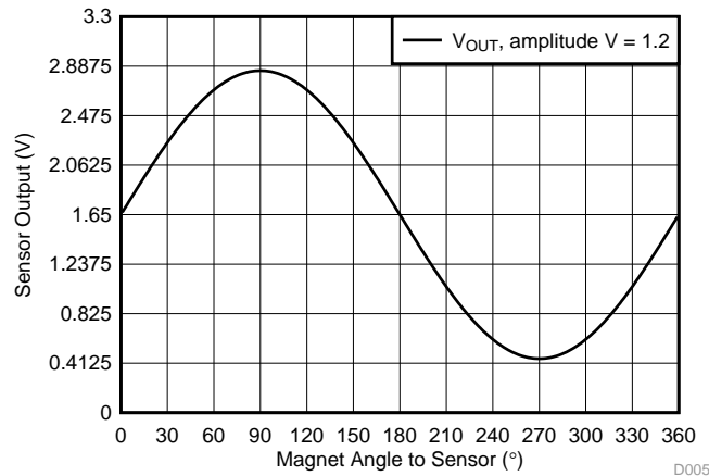
Figure 15. One Sensor Peak Calibrated Data
