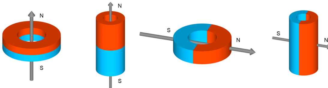
Figure 2. Ring Magnets
