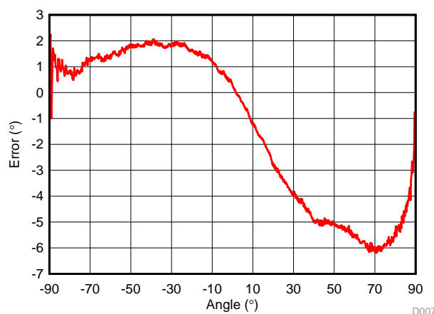
Figure 16. One Sensor Peak Calibrated Error
