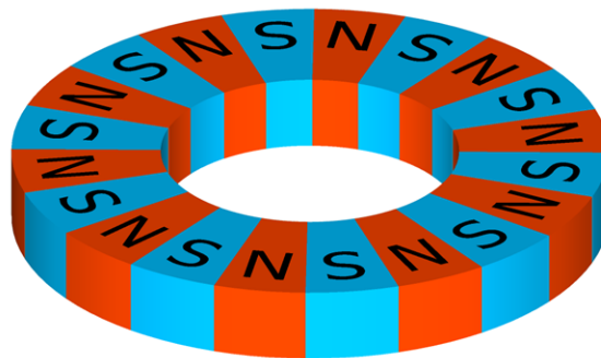
Figure 5. Multipole Ring Magnet
