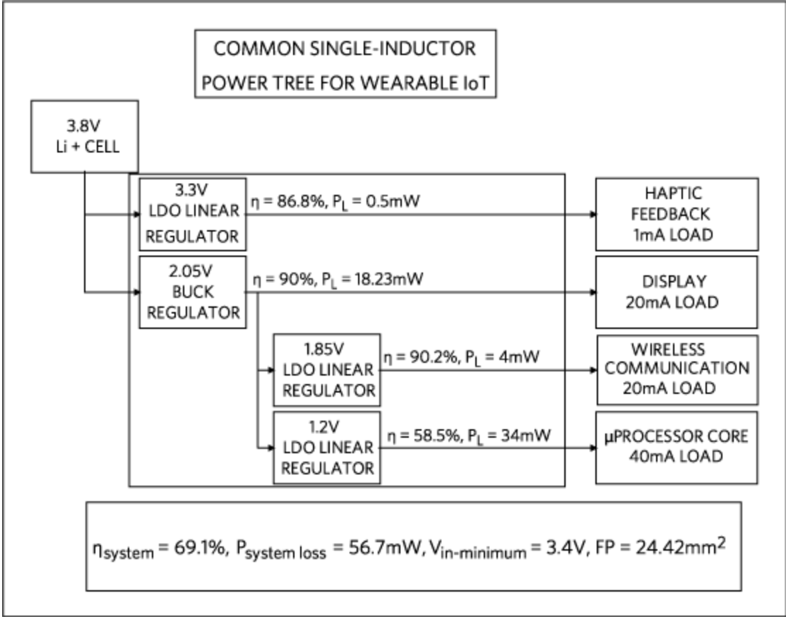
Figure 1. Common single-inductor power tree using a typical PMIC.
