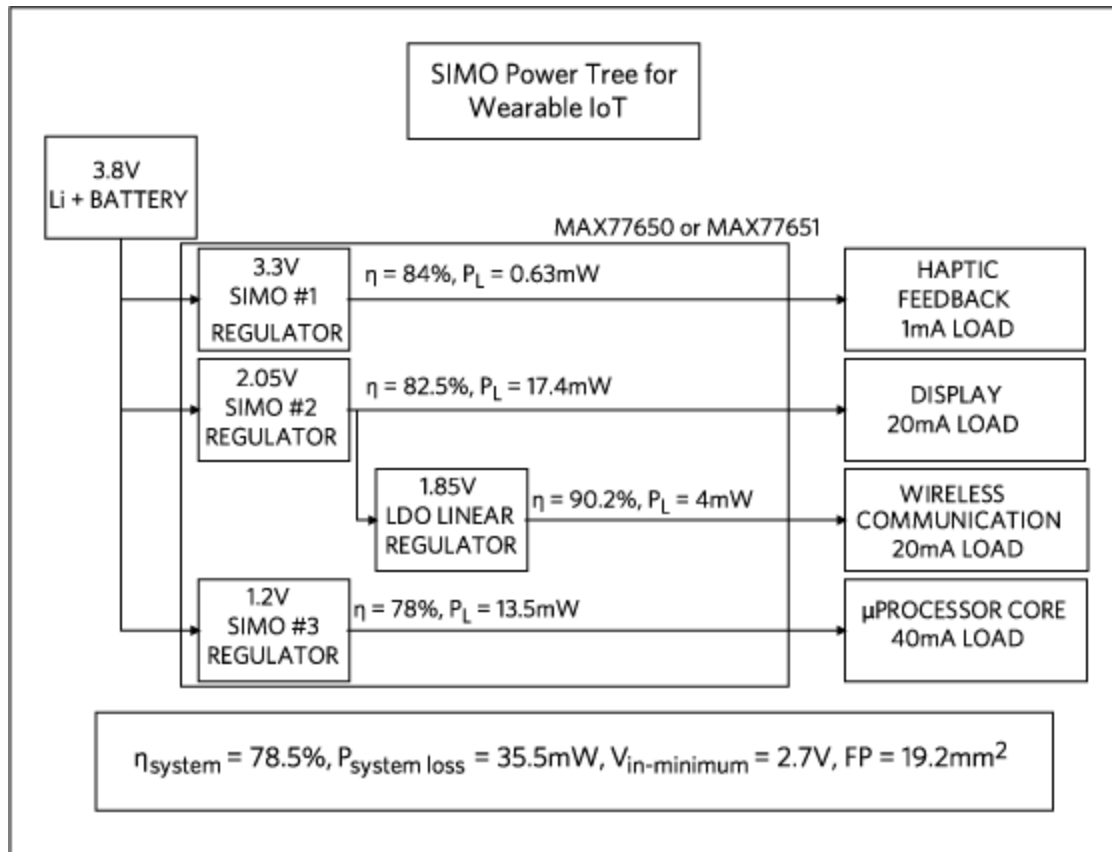
Figure 3. A SIMO power tree using the MAX77650/1 PMIC.
